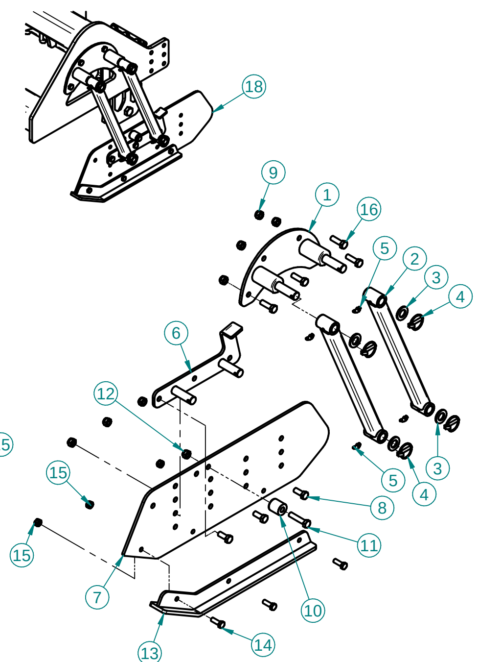
KM & KH Side guard RH
