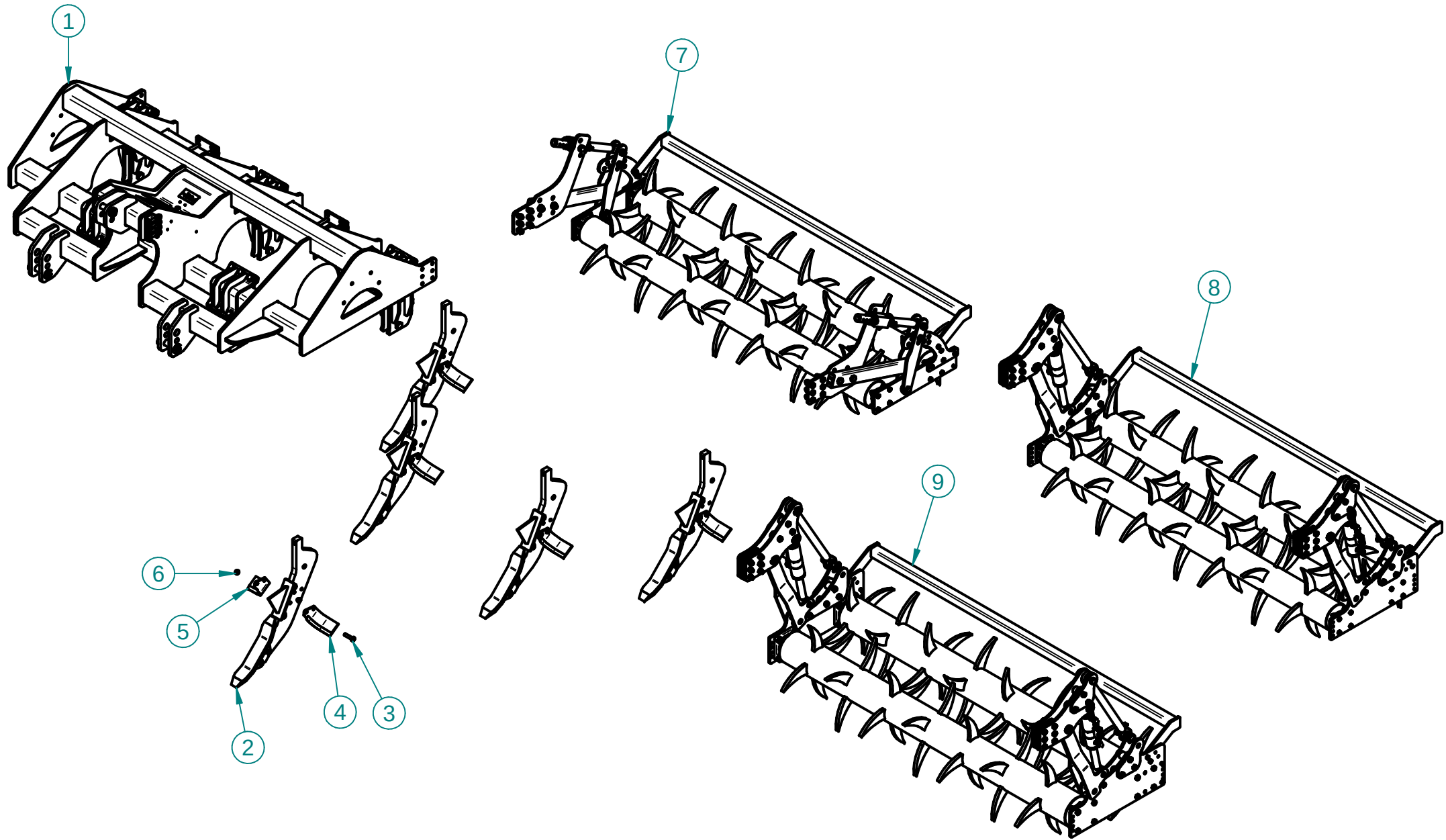
KH Frame Bracket & Rollers
