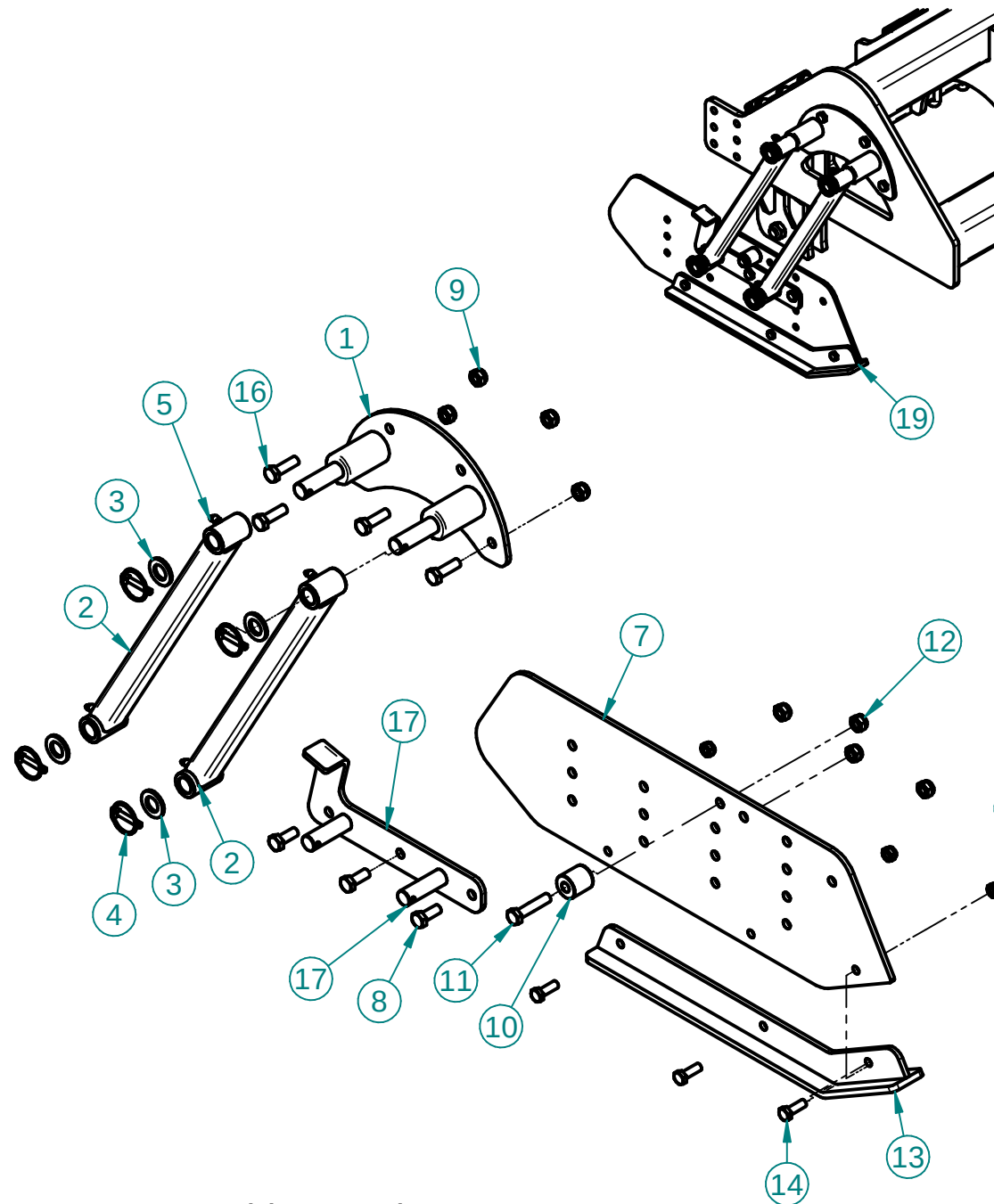
KM & KH Side guard LH
