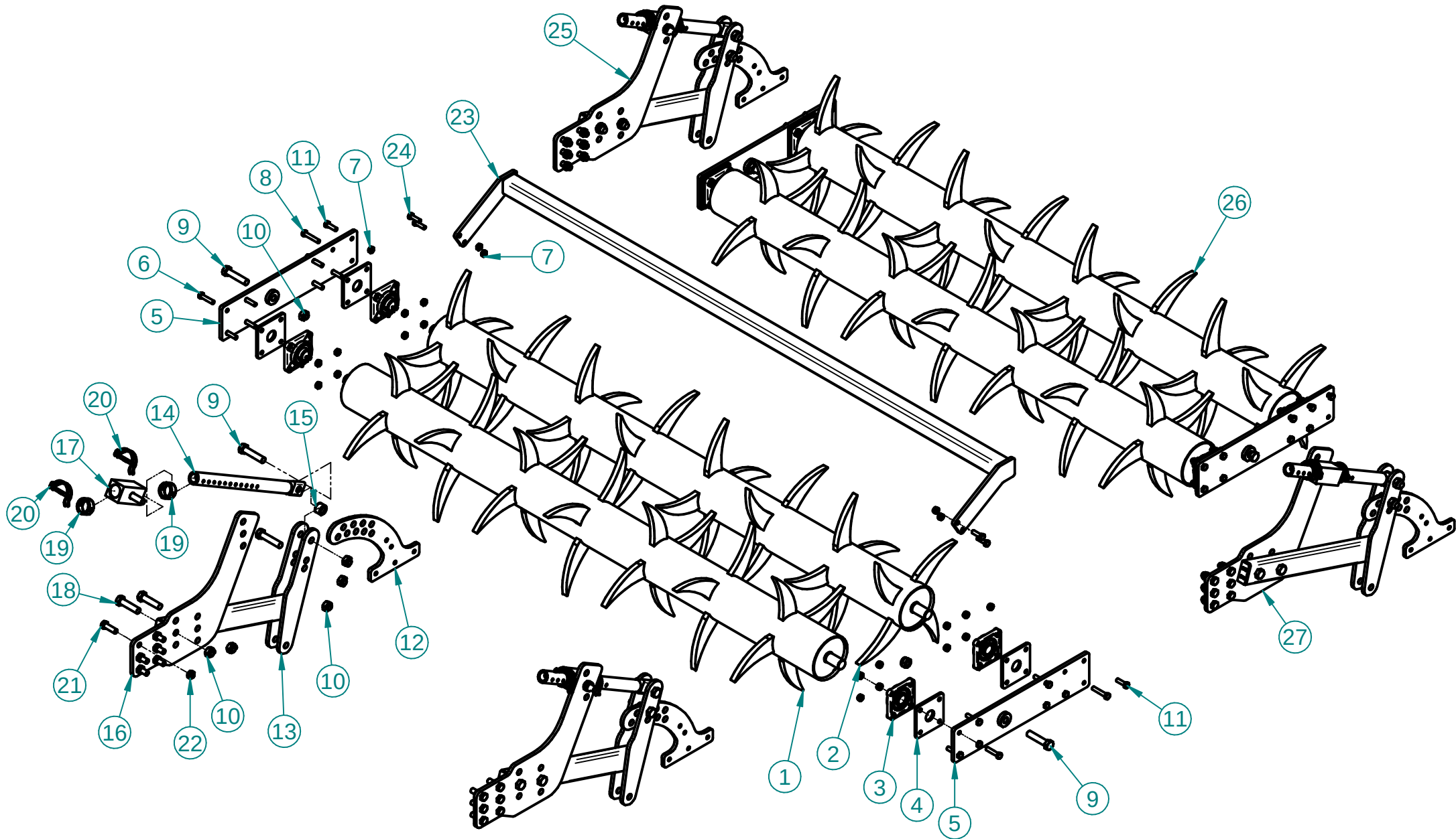
KM & KH Mechanical Roller
