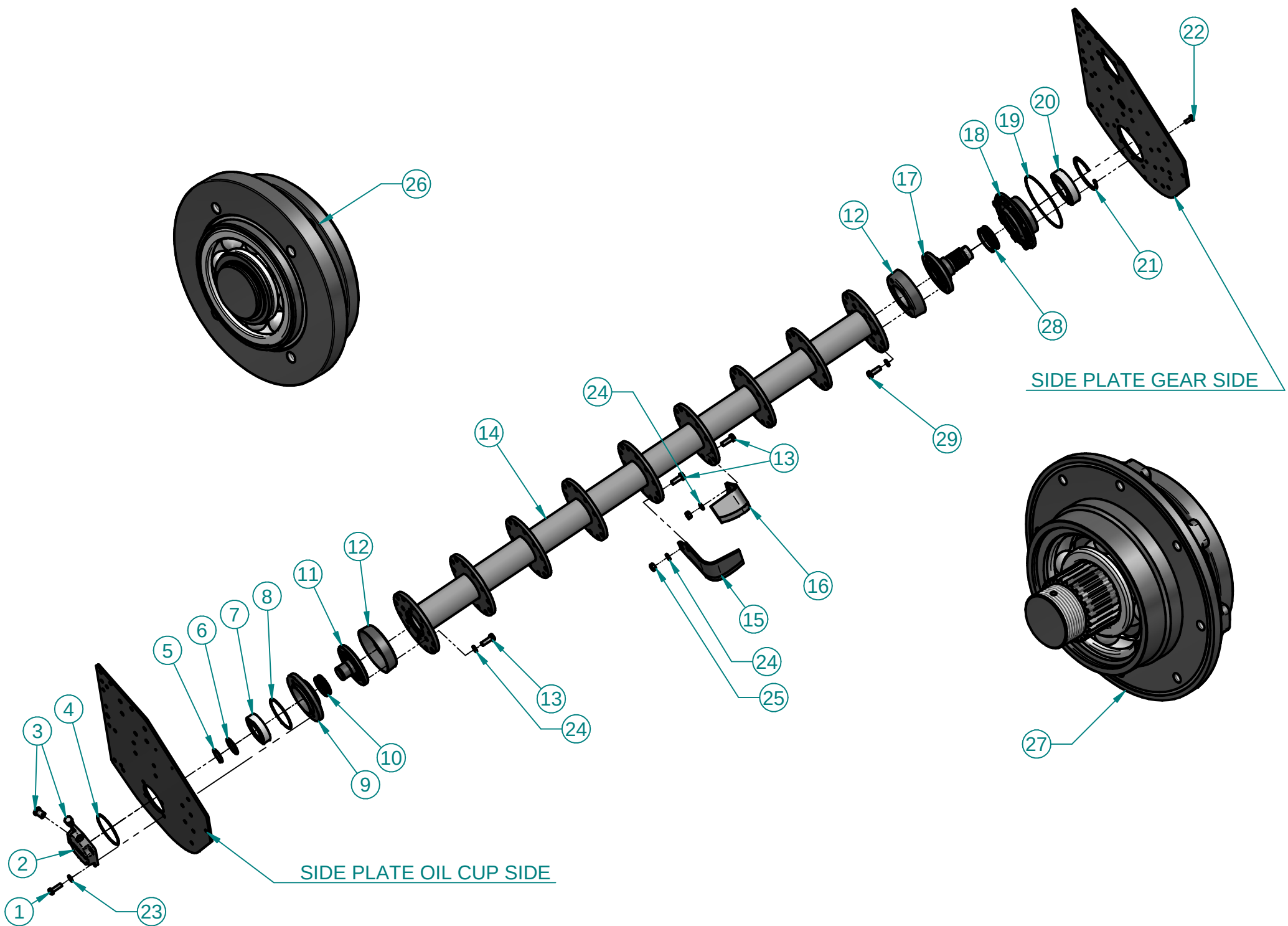
MB Std Rotor Part List
