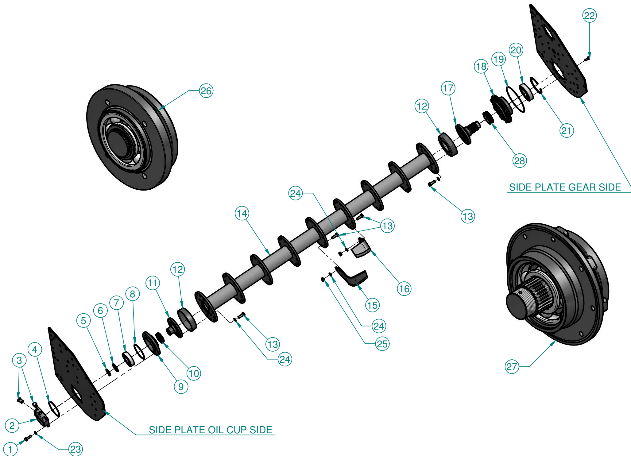
Maximo Std Rotor Part List
